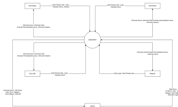
Gambar 1. Context Diagram
